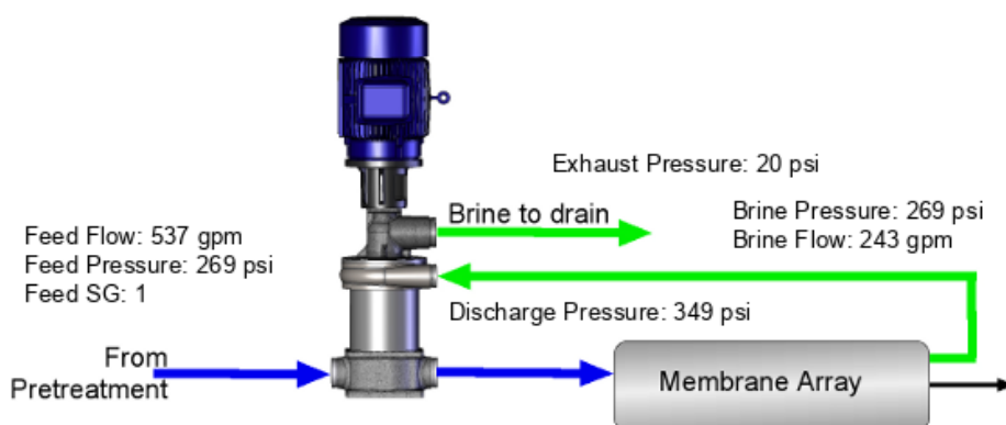
Figure for hydraulic illustration only
